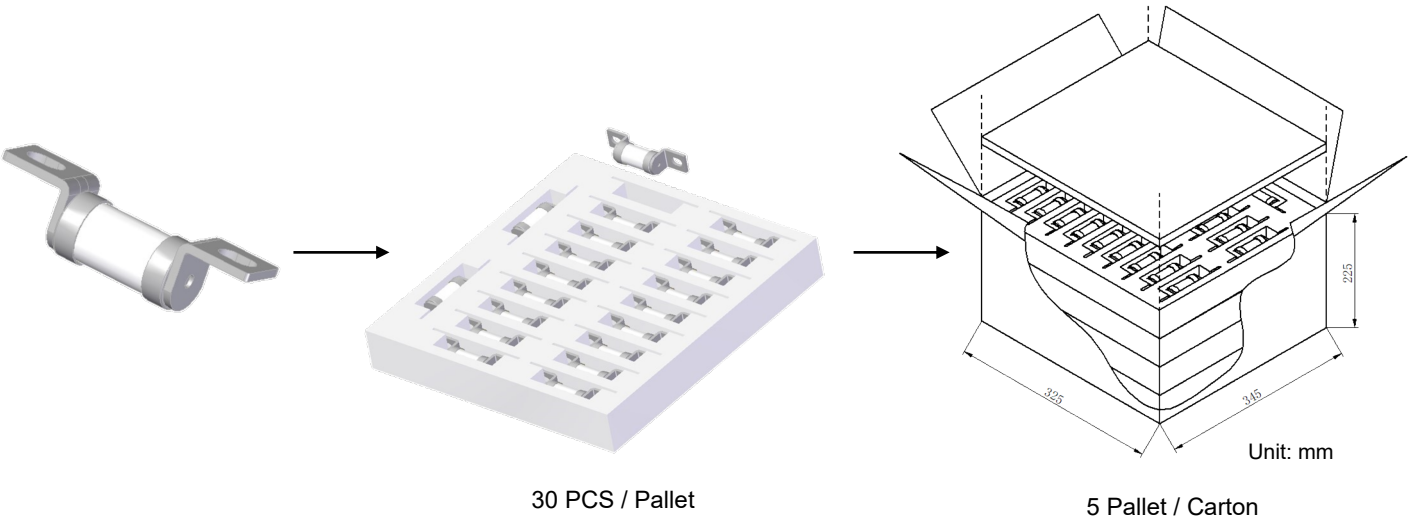
Packaging Drawing:
